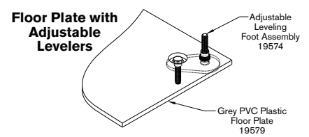
3. Floor Plate & Leveling Feet
