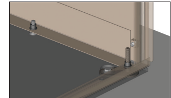
3. Floor Plate & Leveling Feet
